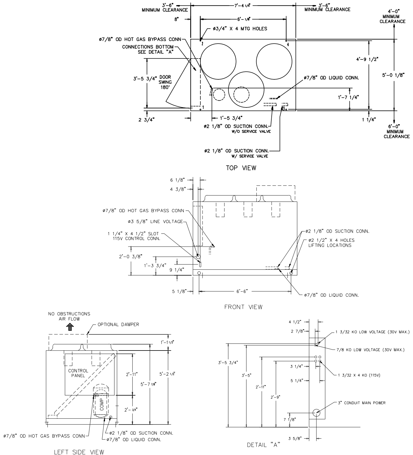
Figure DD-2 –Air-Cooled Condensing Unit –RAUC 25 Ton
